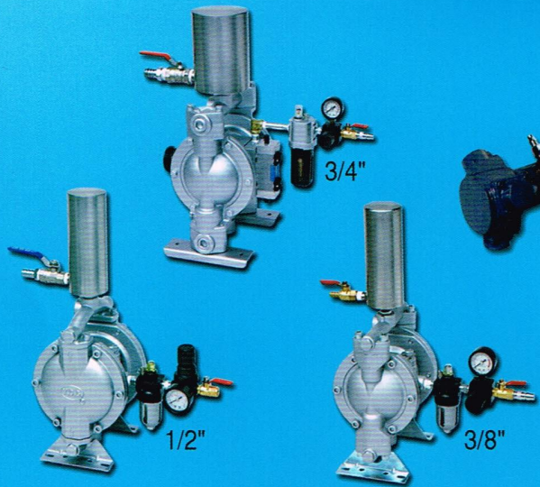
Portable Twin Diaphragm Pump (as for the fluid orifice: 3/8", 1/2", 3/4", 1" etc)
